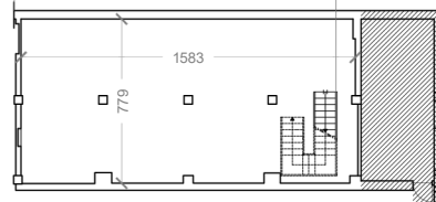
Basement Plan
