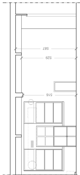
Section AA'
