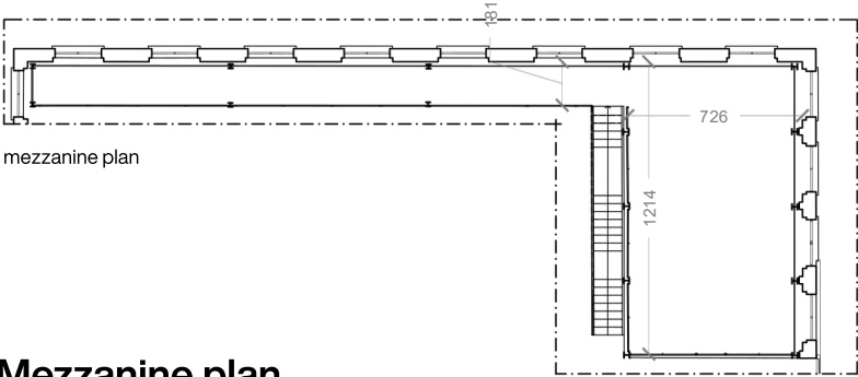
Mezzanine plan
