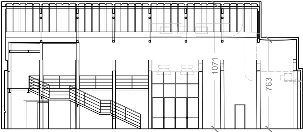
section FF'
