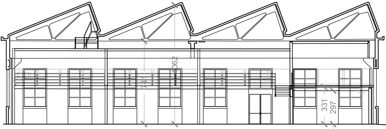
section EE'
