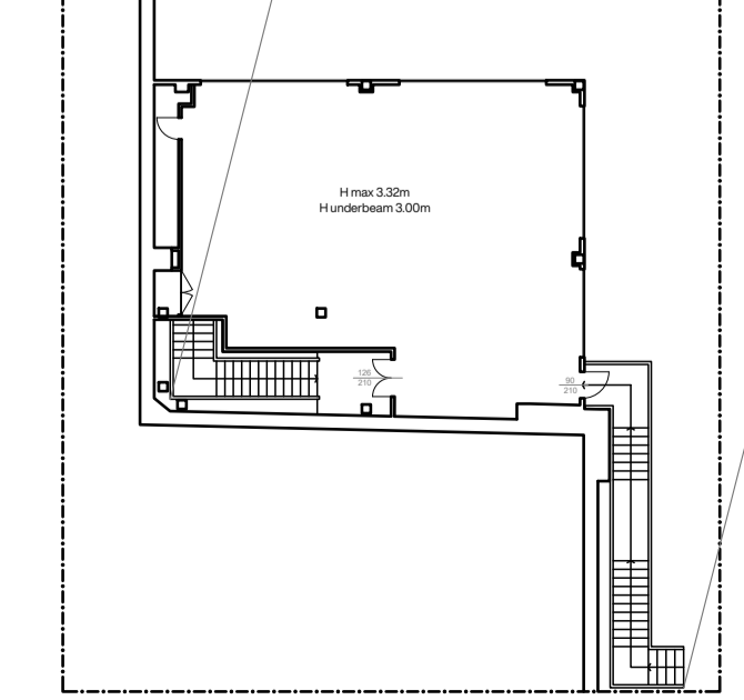
VISION ROOM first floor plan
