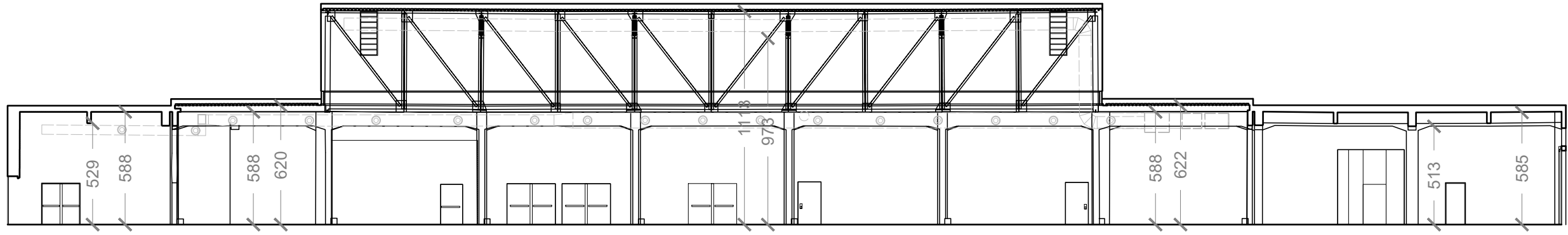
section DD'
